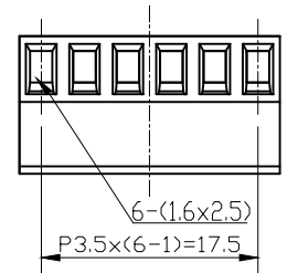
K1 Details Scale=2/1
